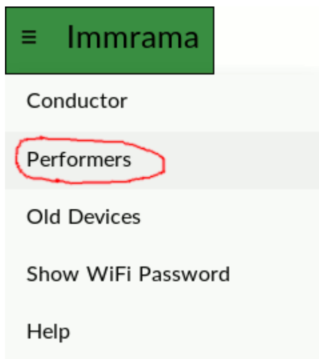
Figure 3: Dropdown menu
